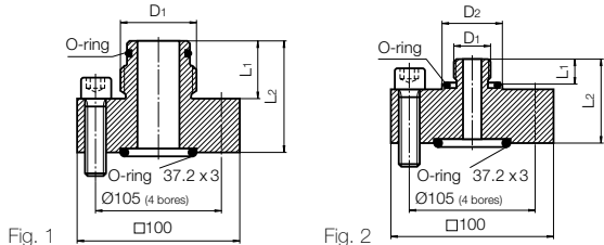
Adapter fittings for accumulator connection S
