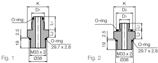
Adapter fittings for accumulator connection S
