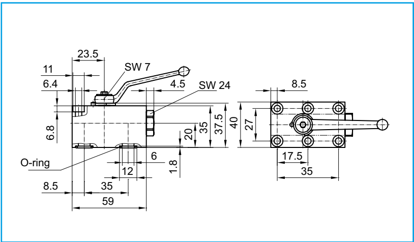
Bypass-ball valve for DN 64 and DN 76
