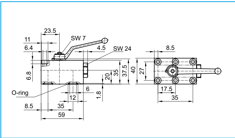
Bypass-ball valve for DN 64 – DN 127
