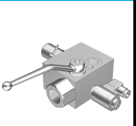
Accumulator safety blocks
