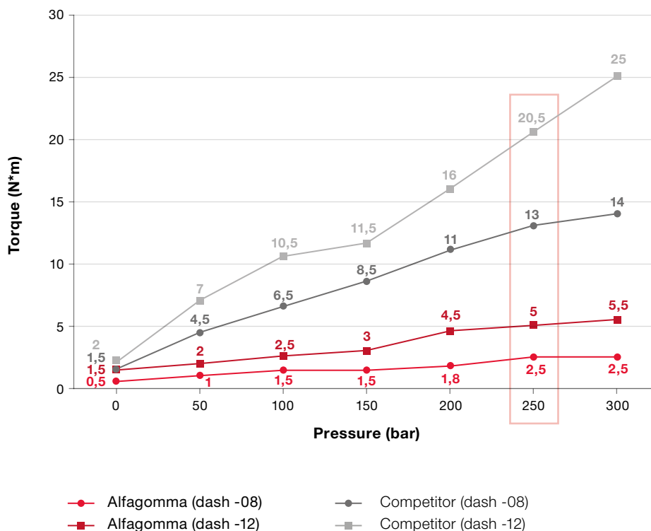
Swivel Connector rotating torque comparison chart Alfagomma versus Competitor
