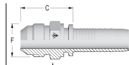
ULKOKIERRE JIC 37° 500200-XX-XX
