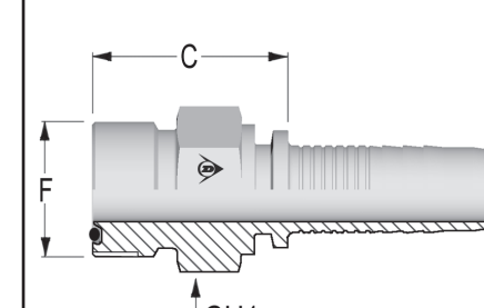
ULKOKIERRE ORFS 50A290-XX-XX
