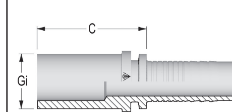
PUTKIJATKEET RSL/RSS - DIN 2353 500930-XX-XX / 500940-XX-XX
