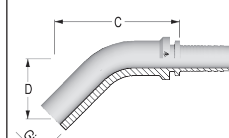
45° PUTKIJATKEET KEVYT RSL/RSS - DIN 2353 509490-XX-XX / 509500-XX-XX
